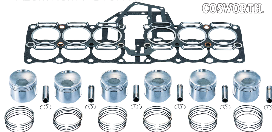
JB-POWER COSWORTH Forged Aluminum Piston Kit φ63 1,328cc ¥ 150,000.-
